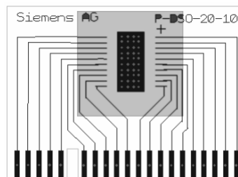
PCB with heat pipes, backside 6 cm 2 cooling area
