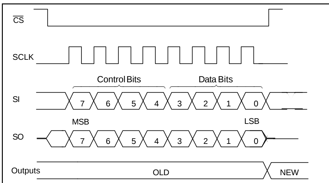
Figure 2: Serial Interface
