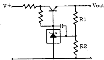
FIGURE 21-SERIES PASS REGULATOR
