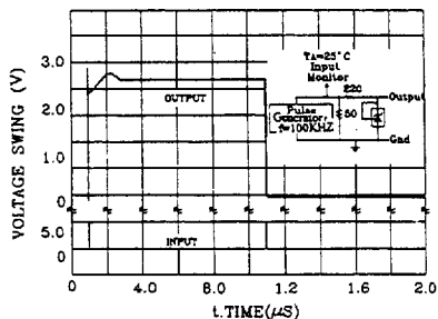
FIGURE 14 - PULSE RESPONSE
