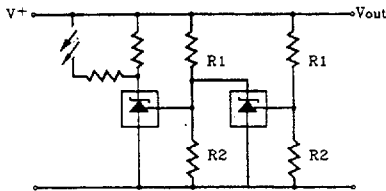
FIGURE 26-VOLTAGE MONITOR
