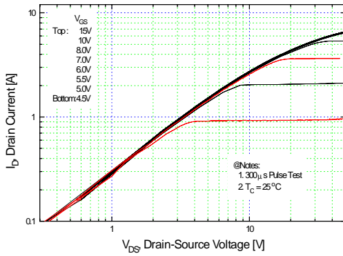
Figure 1. Output Characteristics
