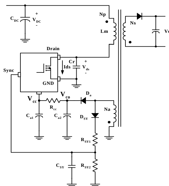
Figure 3. Synchronization circuit
