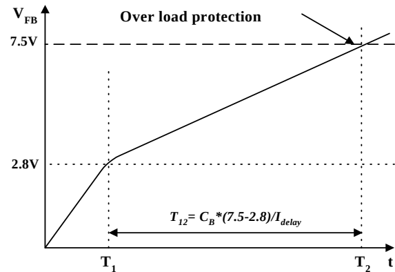
Figure 10. Over load protection
