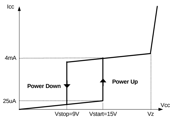
Figure 2. Relation between operating supply current and V cc voltage
