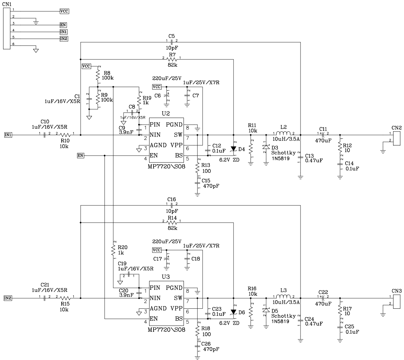
EV0066 / MP7720 Compact Stereo Evaluation Board Schematic ev0066_mp7720_mini_rev_A.sch 8/19/03
