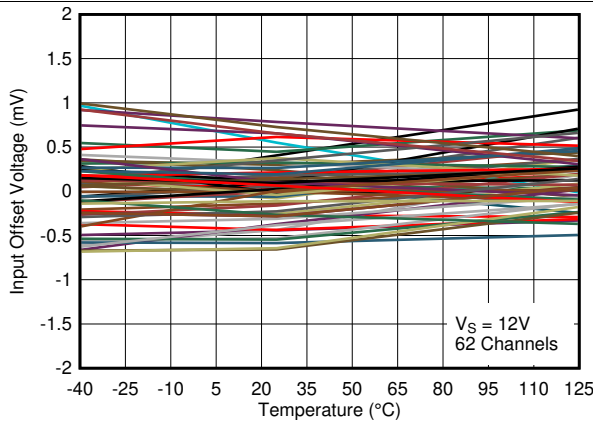
Figure 14. Input Offset Voltage vs. Temperature at 12V
