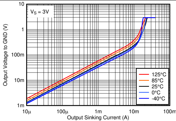
Figure 24. Output Low Voltage vs. Output Sinking Current at 3V
