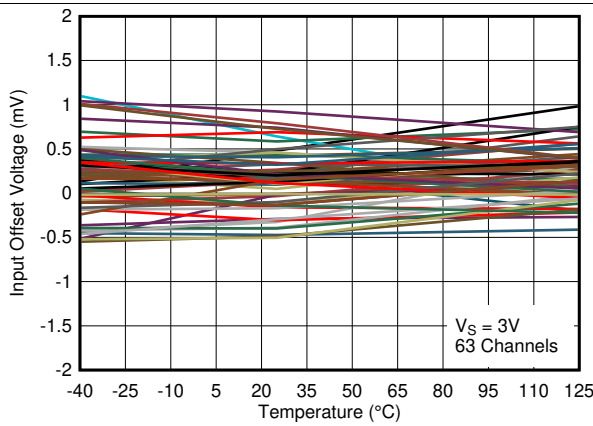
Figure 12. Input Offset Voltage vs. Temperature at 3V
